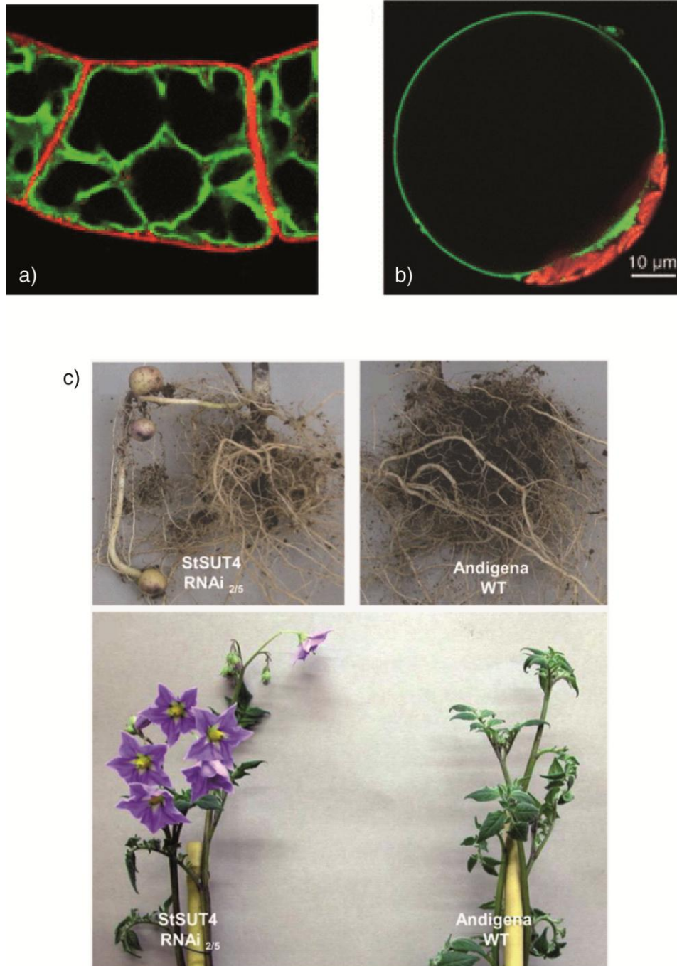
Fig 11. SUT4 clade proteins
