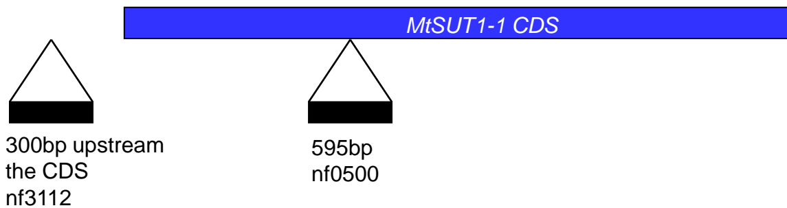
Fig IX.1. Photo and schematic representation of the tnt1 insertion lines in the MtSUT1-1 locus
