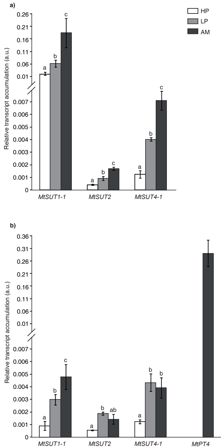
Fig 47. Effect of phosphate nutrition and AMF on transcript level of MtSUT genes
