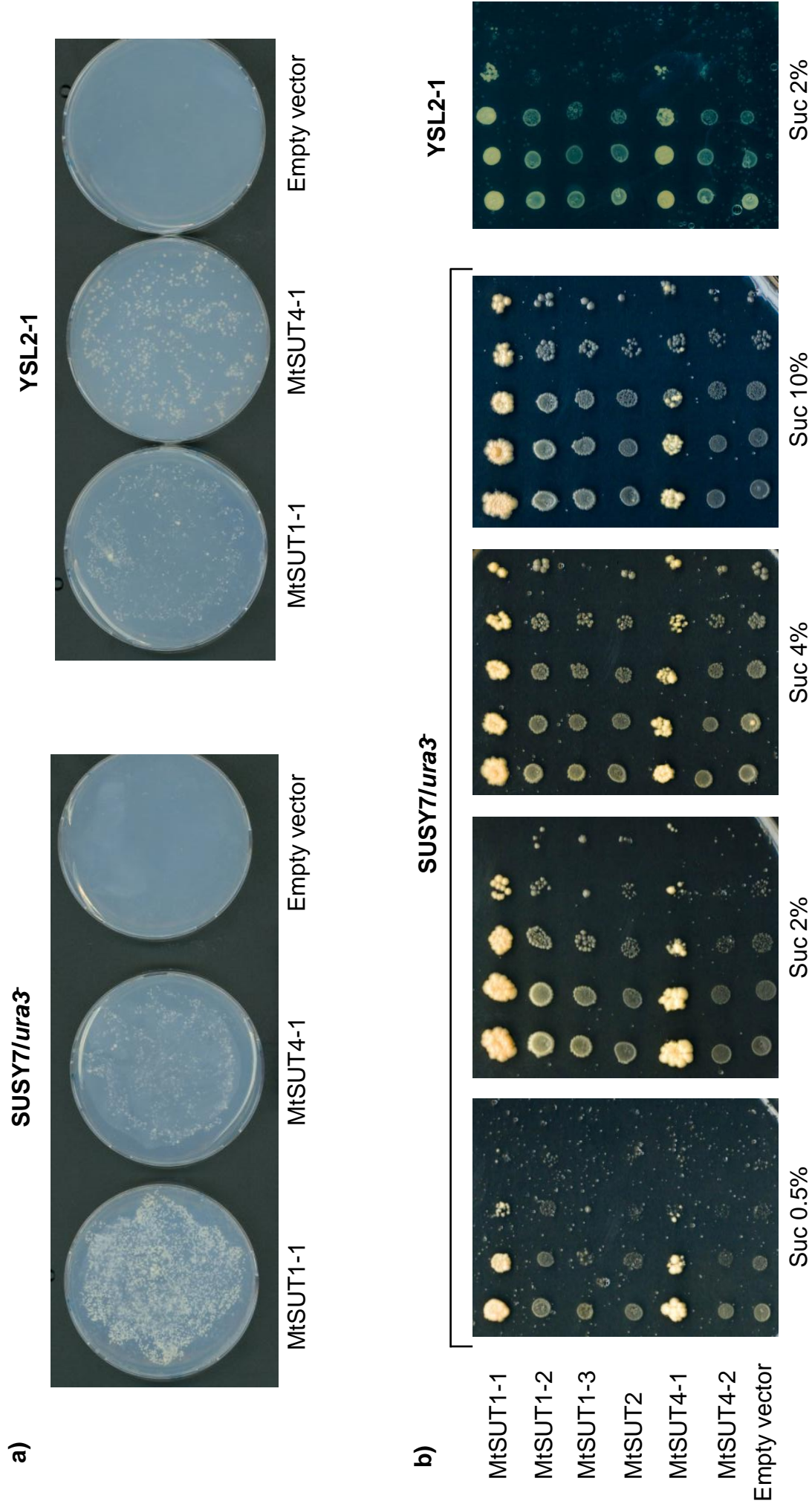
Fig 41. Functional complementation of MtSUTs
