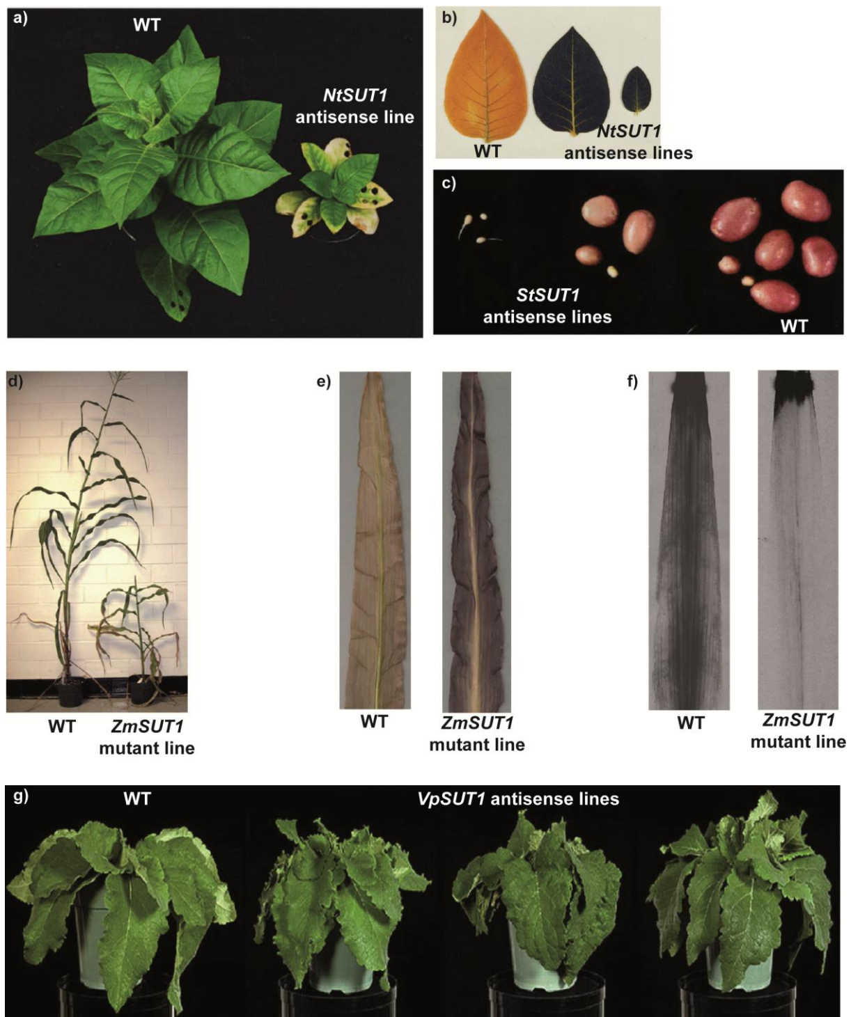
Fig 9. A single SUT protein is necessary for phloem loading in apoplastic loader plants
