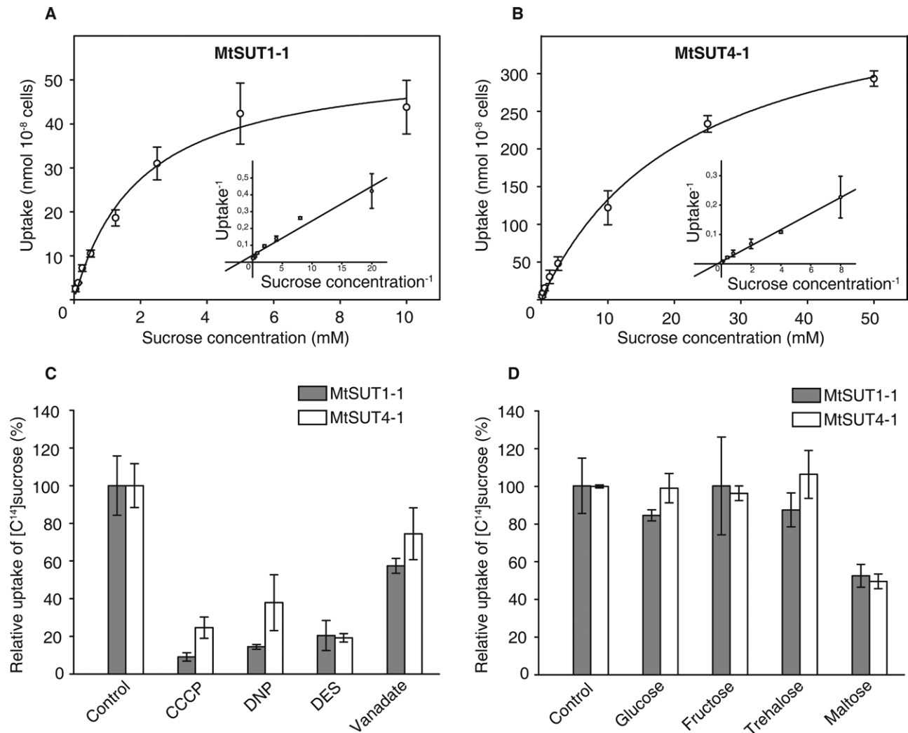
Figure 3. Biochemical Characterization of MtSUT1-1 and MtSUT4-1 .
