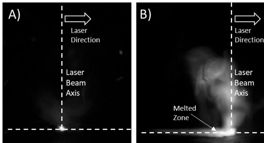
Figure 50. Vapor plumes (side view) of A) A5754 captured with 520 \mu s exposure time and B) Ti captured with 10 \mu s exposure time (Laser power:3 kW, Welding speed: 3 m/s).
