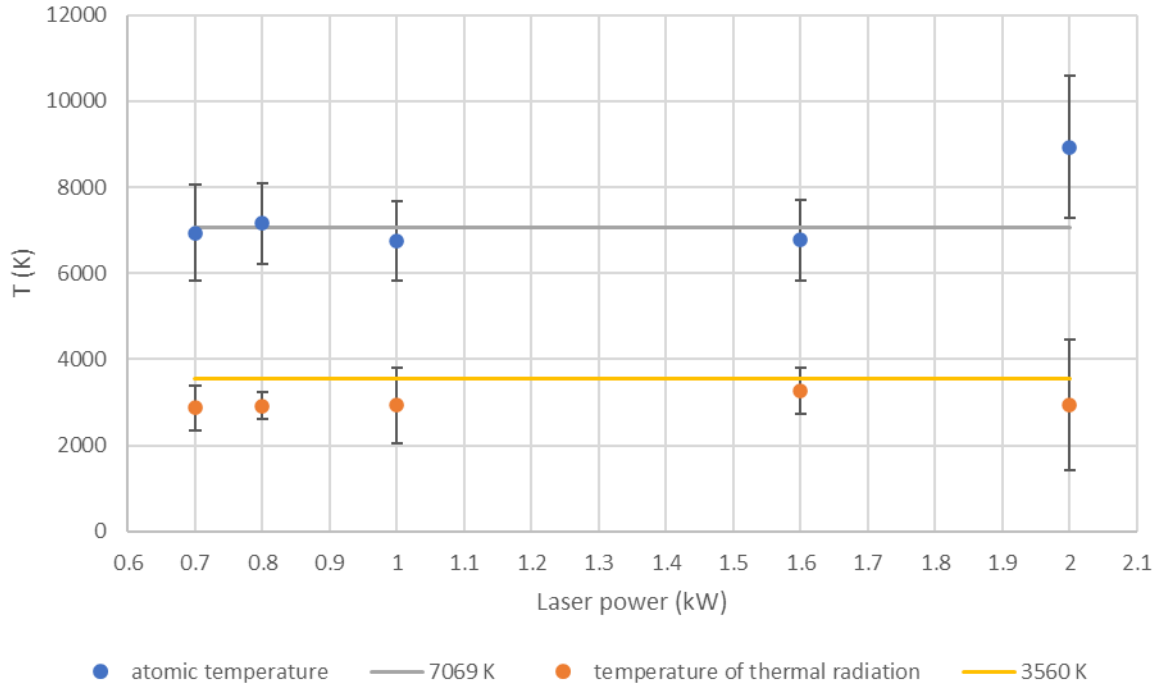
Figure 133. Evolution of Titanium Temperatures as a Function of Power ( 3\sigma bar)
