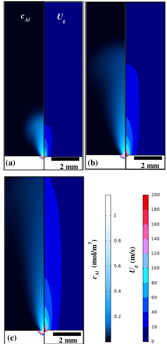
Figure 8. The calculated concentration of Al atoms in the gas phase (on the left) and gas velocity field (on the right) at pulse times of (a) 468 \mu\text{s} , (b) 936 \mu\text{s} and (c) 1404 \mu\text{s} .
