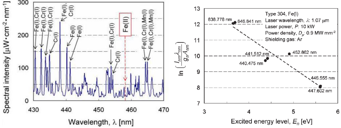
Figure 23. Emission spectra of the vapor plume for 10kW fiber laser welding of 304 stainless steel within 430-470 nm and the corresponding Boltzmann plots [161].
