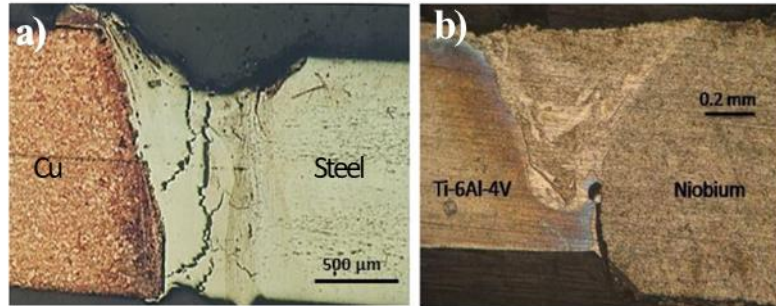
Figure 16. Post-mortem images of the melted zone development in a) Cu/Steel [139] and b) Ti-6Al-4V/Niobium [138].
