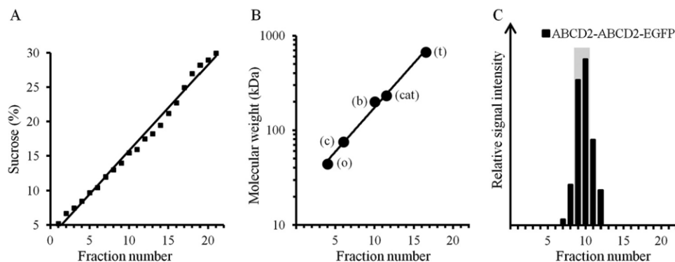
Figure 1. Calibration of velocity sucrose gradients with soluble and membrane protein markers. A , 5–30% (w/v) sucrose gradient linearity was checked by monitoring of sucrose concentration using a refractometer. Fractions 1–22 correspond to fractions from the top to the bottom of the gradient. B , calibration curve was drawn from the flotation of native soluble protein markers ( t , thyroglobulin (669 kDa); cat , catalase (232 kDa); b , \beta -amylase (200 kDa); c , conalbumin (75 kDa); o , ovalbumin (44 kDa)) in parallel and equivalent sucrose gradients. C , ABCD2-ABCD2-EGFP (194 kDa) solubilized with 1% SDS, used as a membrane protein size marker, floated in fractions 9 and 10 (indicated by a gray bar) as monitored by densitometry analysis of immunoblotting performed with an anti-GFP antibody for all collected fractions.
